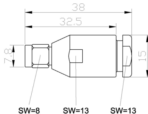
Alle Angaben in mm / All dimensions are in mm Pin: Loch / hole: \varnothing 2 mm
