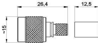
All dimensions in mm - Alle Dimensionen in mm
