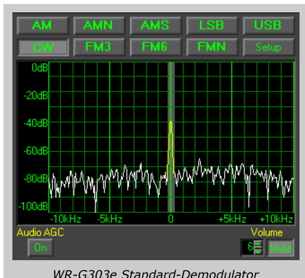
WR-G303e Standard-Demodulator
