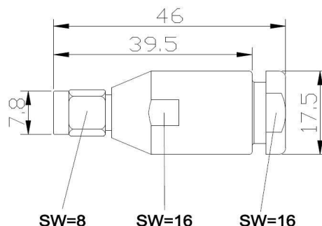
All dimensions in mm SMA-Connector ECOFLEX 10 Part NO.7362
